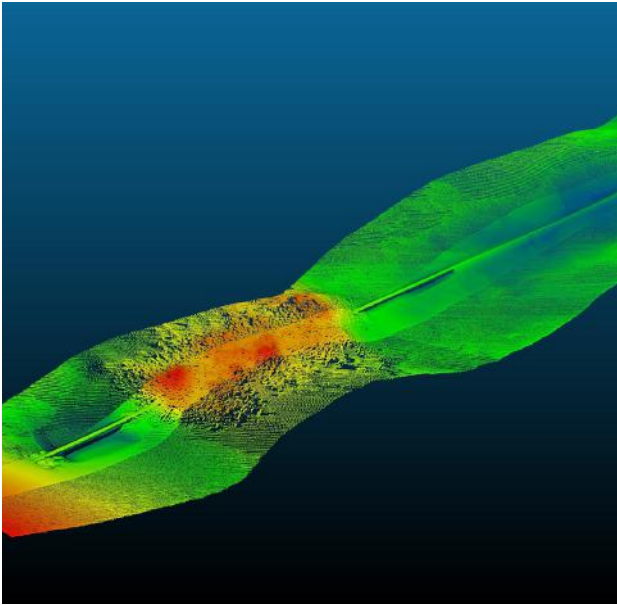
Pipeline Image captured with UHD. Image courtesy of Swathe Services
