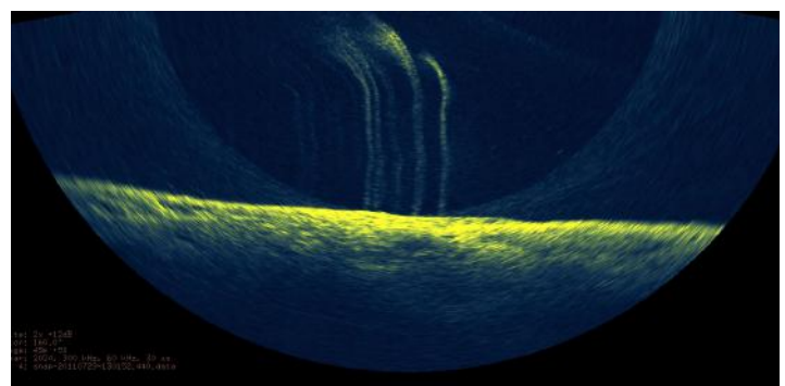
Image captures with FLS. Courtesy of GEOMAR Helmholtz Center for Ocean Research
