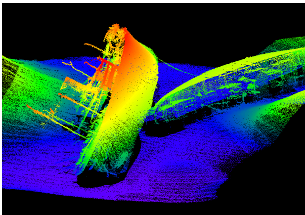
Image captured with UHR. Courtesy of Tim Shaw, CSA
