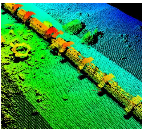
Image captured with Pipeline Mode Courtesy of DOFSubsea
